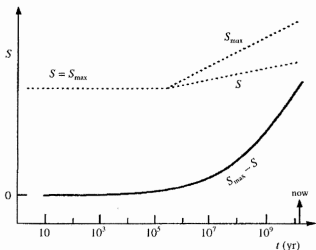
Fig. 2.4. In the expanding Universe, the actual entropy, S , increases less rapidly than the maximum possible entropy, S_{\max} , once the symmetry of equilibrium broke when matter and radiation decoupled at \sim 10^5 years. By contrast, in the early, equilibrated Universe, S = S_{\max} for the prevailing conditions. The potential for the growth of order – (S_{\max} - S) , shown as the thick black curve – has increased ever since the start of the Matter Era. Accordingly, the expansion of the Universe can be judged as the ultimate source of free energy, promoting the evolution of order in the cosmos. This potential rise of order compares well with the family of curves of Fig. 2.2 and provides a theoretical basis for the growth of systems complexity
